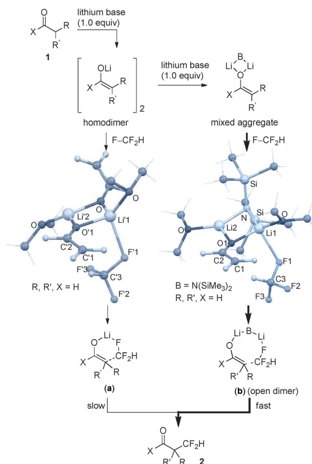
Scheme 3. Plausible mechanism of \alpha -difluoromethylation.
