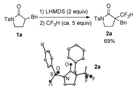
Scheme 2. Direct difluoromethylation of the lithium enolate with fluoroform. Bn = benzyl, Ts = 4-toluenesulfonyl.
