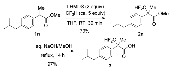
Scheme 4. Synthesis of the \alpha -difluoromethyl analogue of ibuprofen.
