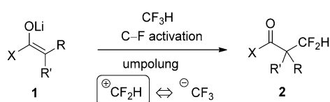
Scheme 1. Umpolung of fluoroform with a lithium enolate.
